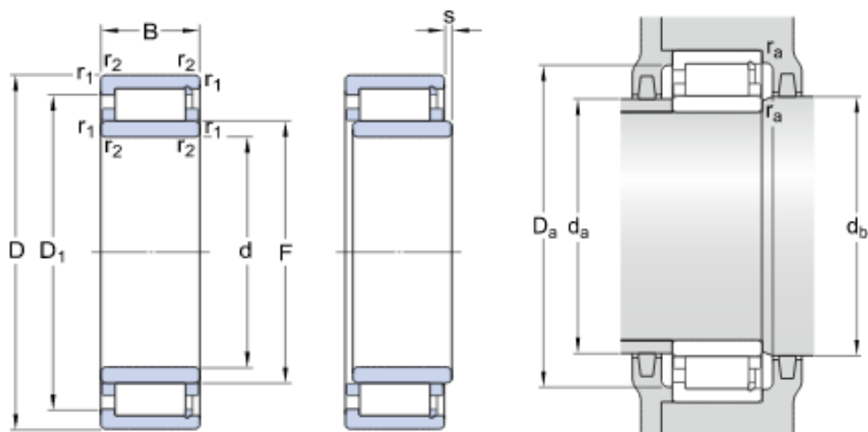
Single Row Cylindrical Roller Bearing
